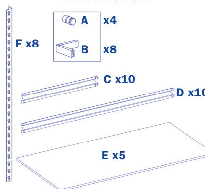
Assembly Option 1
