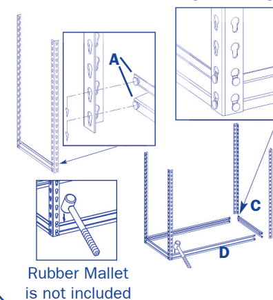
Assembly Option 2
